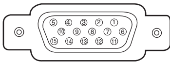
Pin Configuration
